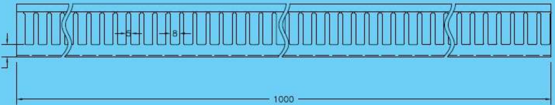
FRONT VIEW
