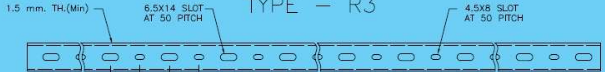
BOTTOM VIEW
