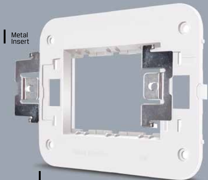
Base Frame
