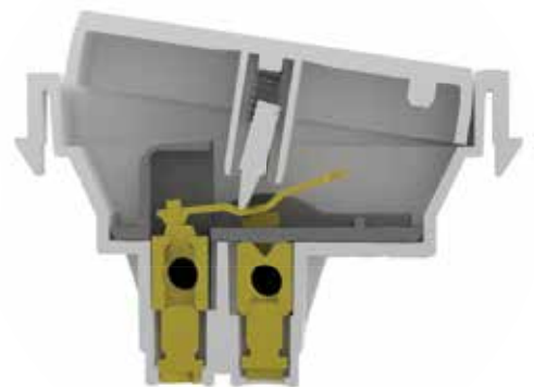
Normal Switch Structure
