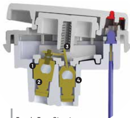
Toggle Type Structure
